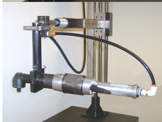
RT. ANGLE NUTRUNNER BM-TT100-FL-RAM
